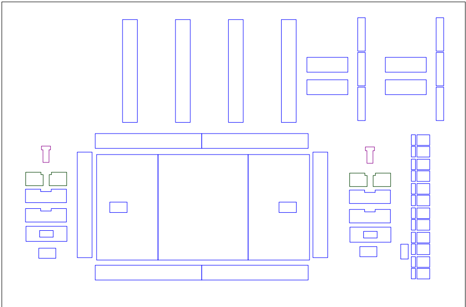
ITEM E.I.I - QTY X 2 - 18MM PLY. 12MM PLY. 12MM UHPPE
