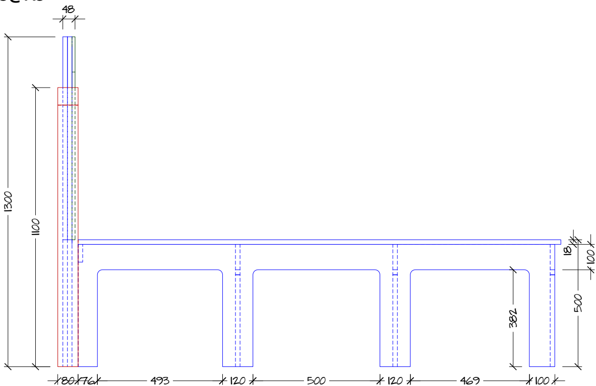
E.3 FRONT VIEW 1:15@A3
