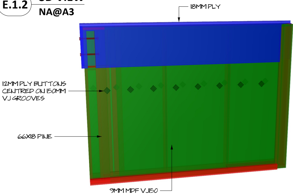
E.1.2 3D VIEW NA@A3
