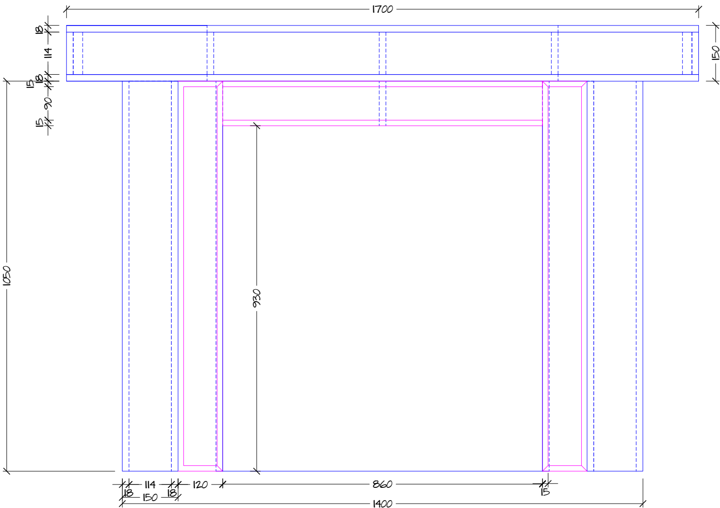
E.4 FRONT VIEW 1:10@A3
