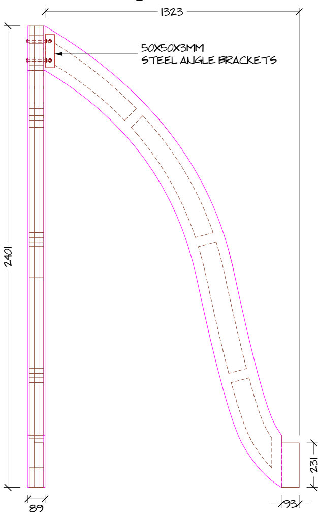
E.1.4 END VIEW 1:20@A3
