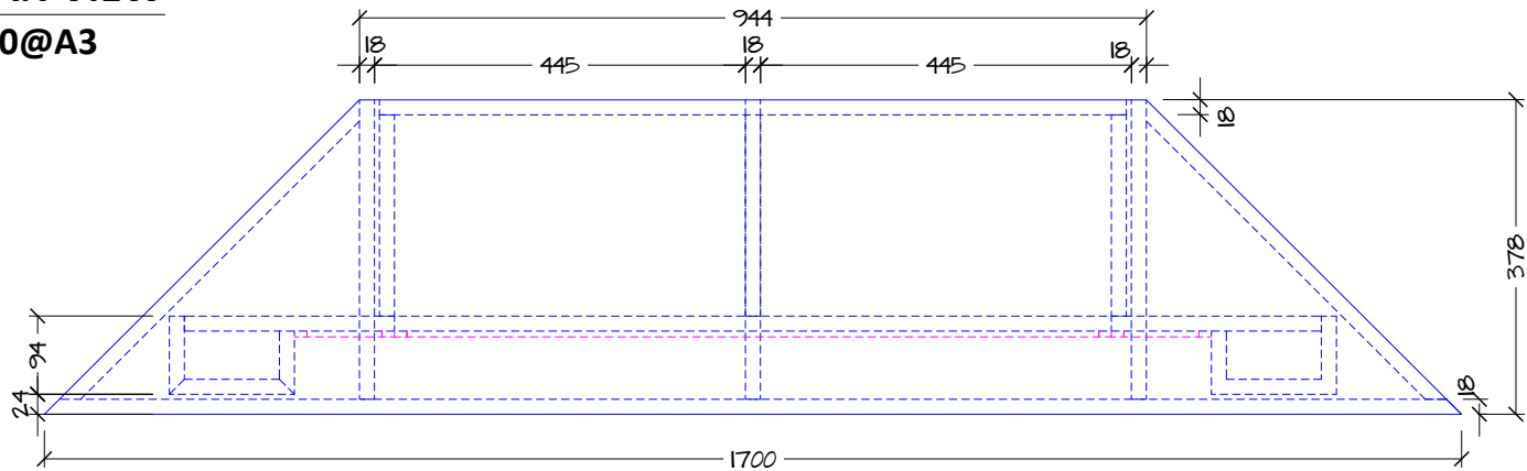
E.4 END VIEW 1:10@A3
