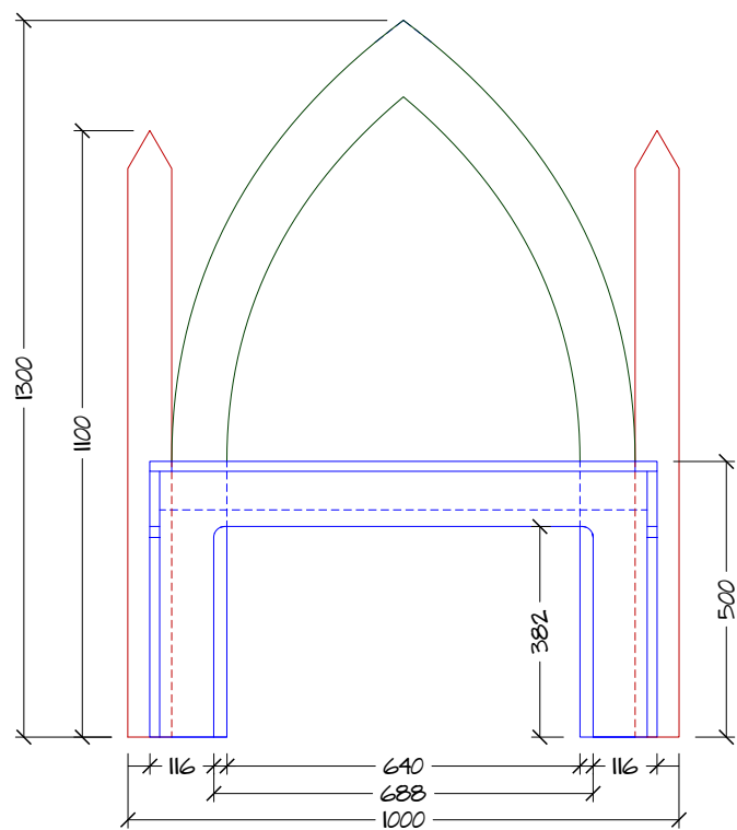
E.3 END VIEW 1:15@A3
