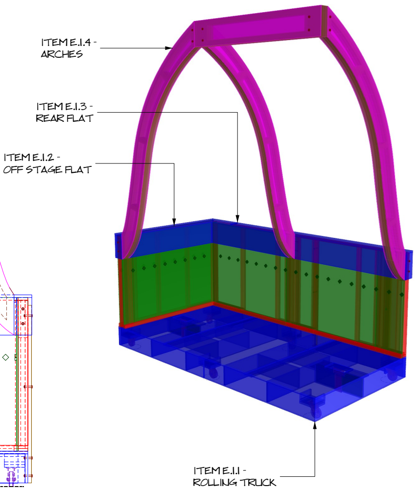
E.1 3D VIEW NA@A3
