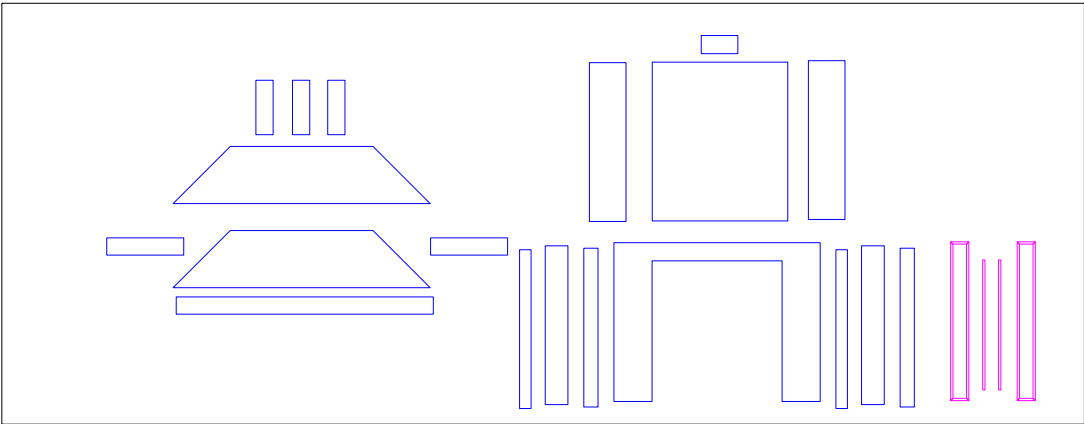
ITEM E.5 - QTY X 1 - 18MM PLY. 7MM PLY.
