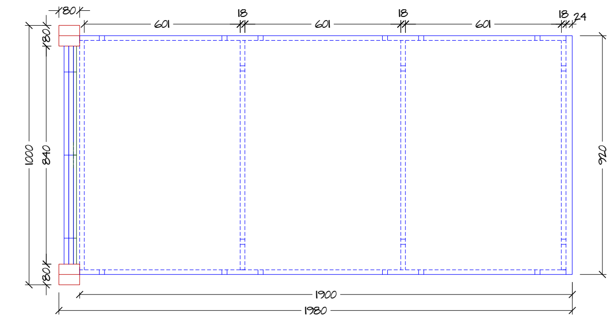
E.3 FRONT VIEW 1:15@A3
