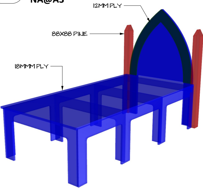
E.3 3D VIEW NA@A3
