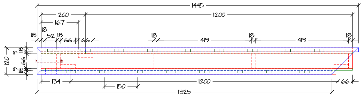
E.1.2 PLAN VIEW 1:10@A3
