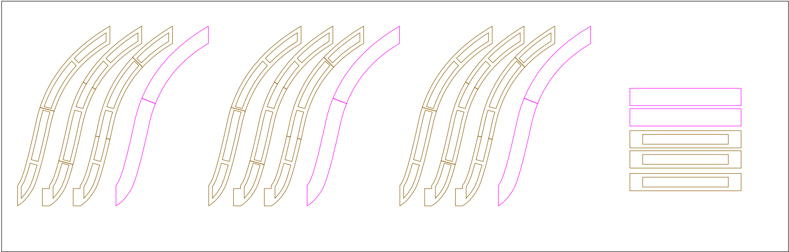
ITEM E.I.4 - QTY X 2 - 25MM PLY. 7MM PLY.
