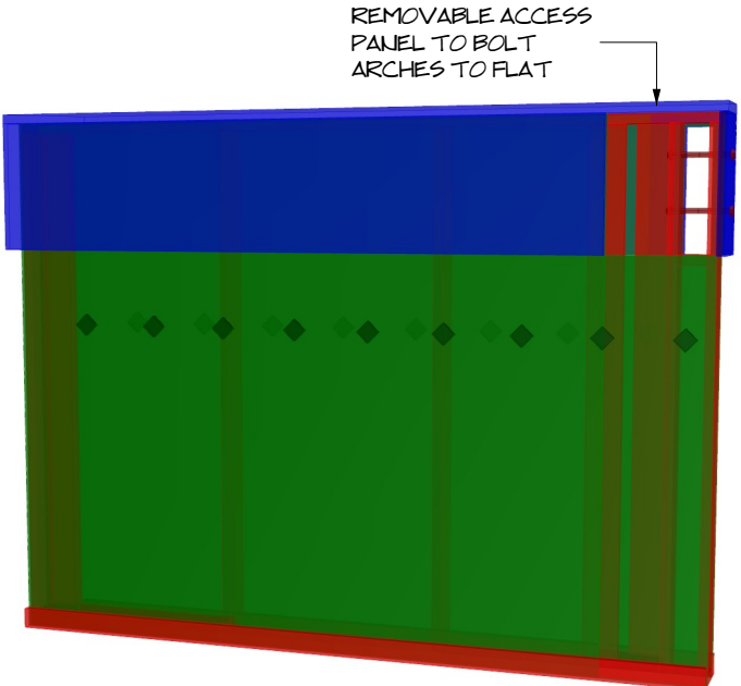
E.1.2 3D VIEW NA@A3
